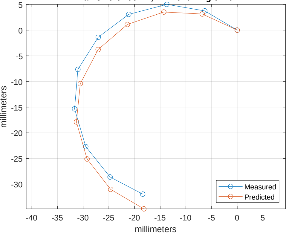
Hainsworth 95A 1, DT Bend Angle Fit
